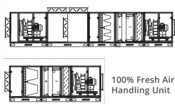
Air Handling Unit with Mixture Cell
