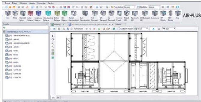
Air Handling Unit with Mixture Cell
